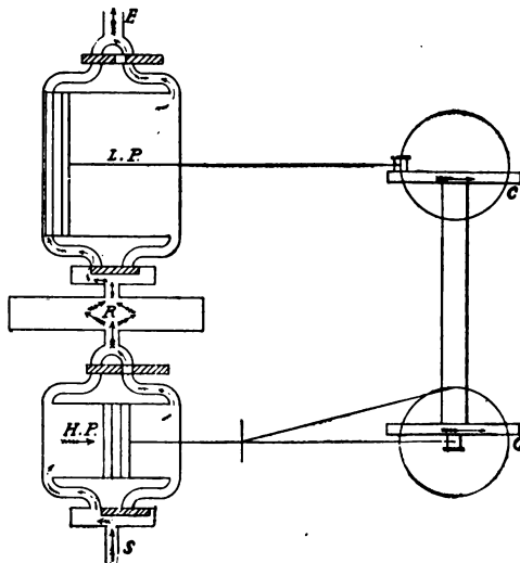
FIG. 333.—Diagram of a "Cross Compound" Steam Engine. The cranks, C and C, are at 90°. The high-pressure steam port is at S; the H. P. exhaust to L. P. cylinder at R, and the exhaust to atmosphere from the low-pressure cylinder, at E.
